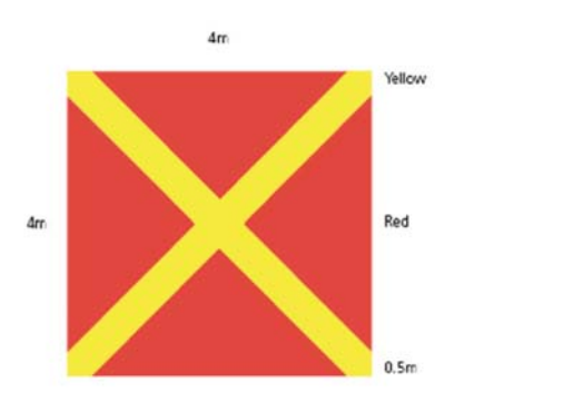
Helideck Closed Marker Marker 4 x 4 mtr
